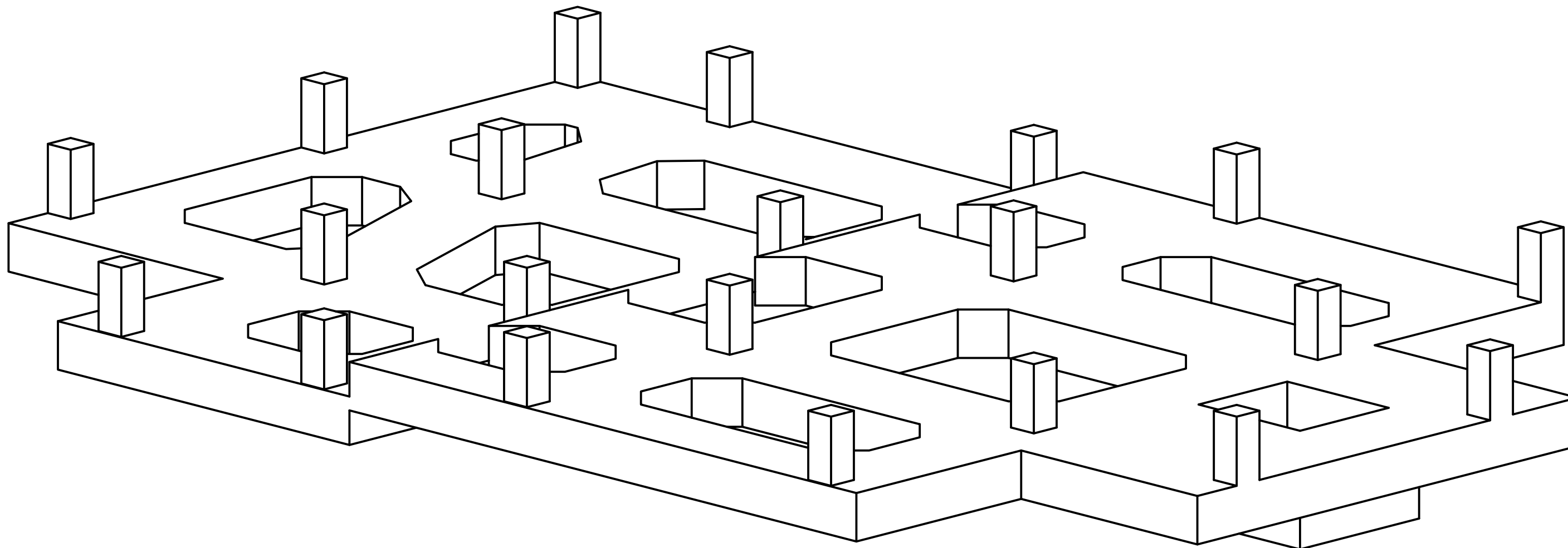
Foundation 3D-View Concrete Volume : 159.5 m3
