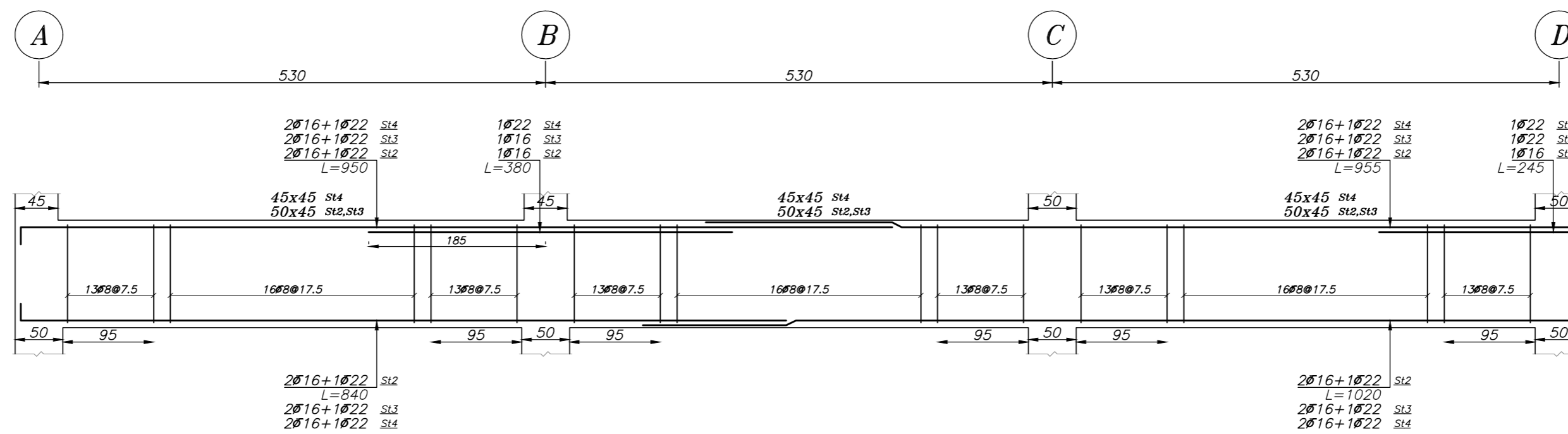
Beam Typ. B-2 Elev: 1110,1440,1770 H Scale 1:50 V Scale 1:20
